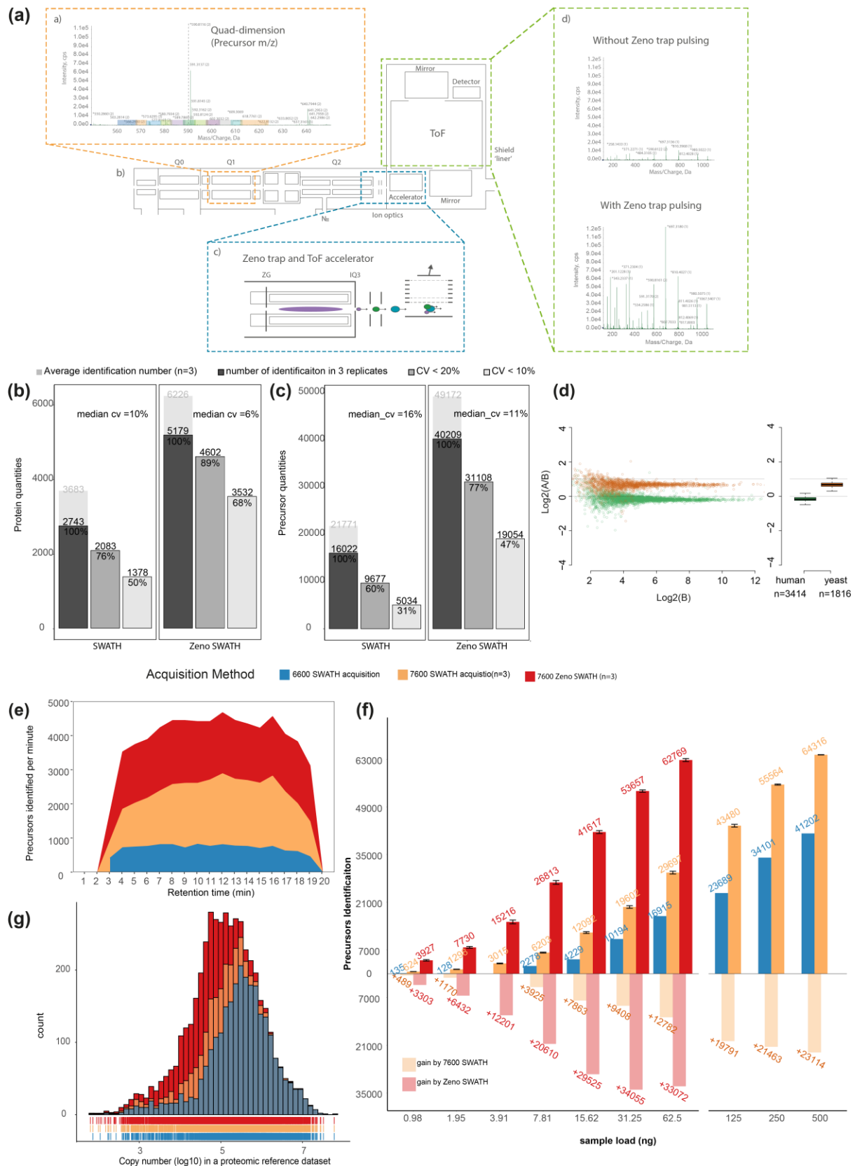
Figure 1. Zeno SWATH and its performance on K562 using 5 \mu l/min, 20 min micro-flow chromatography.
